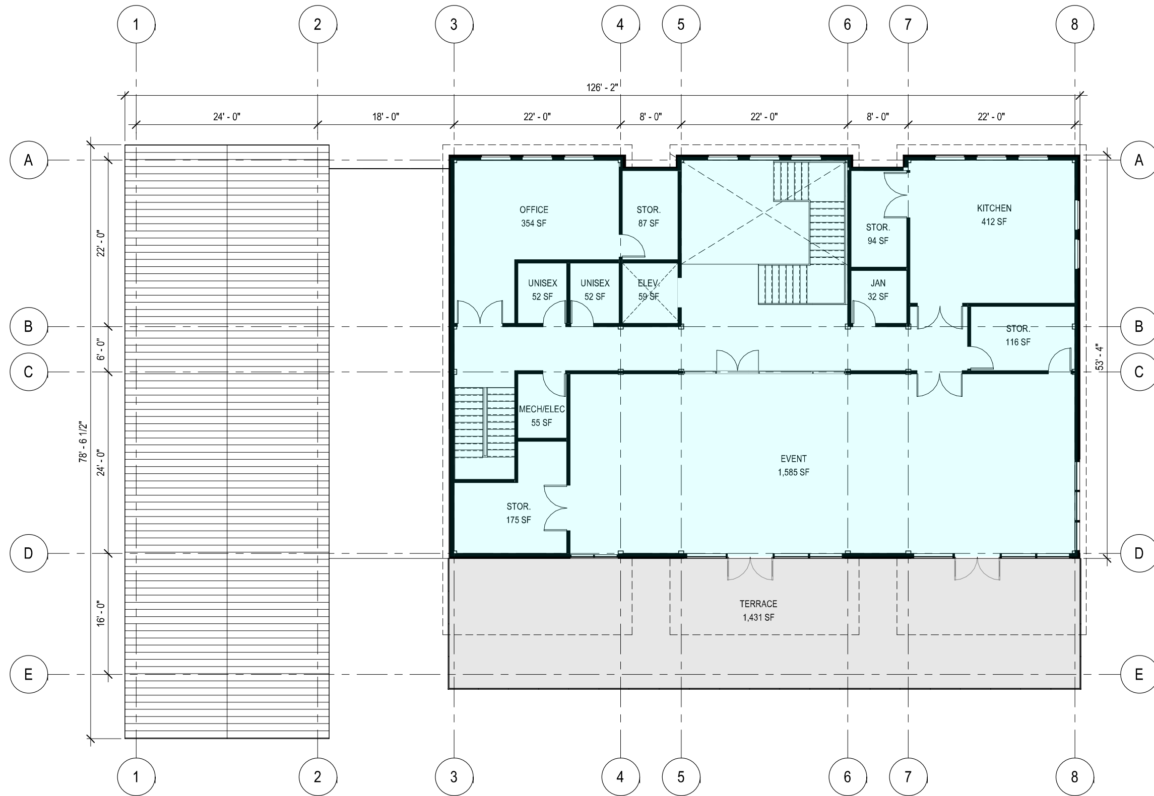
Floor Plan - Level 2
