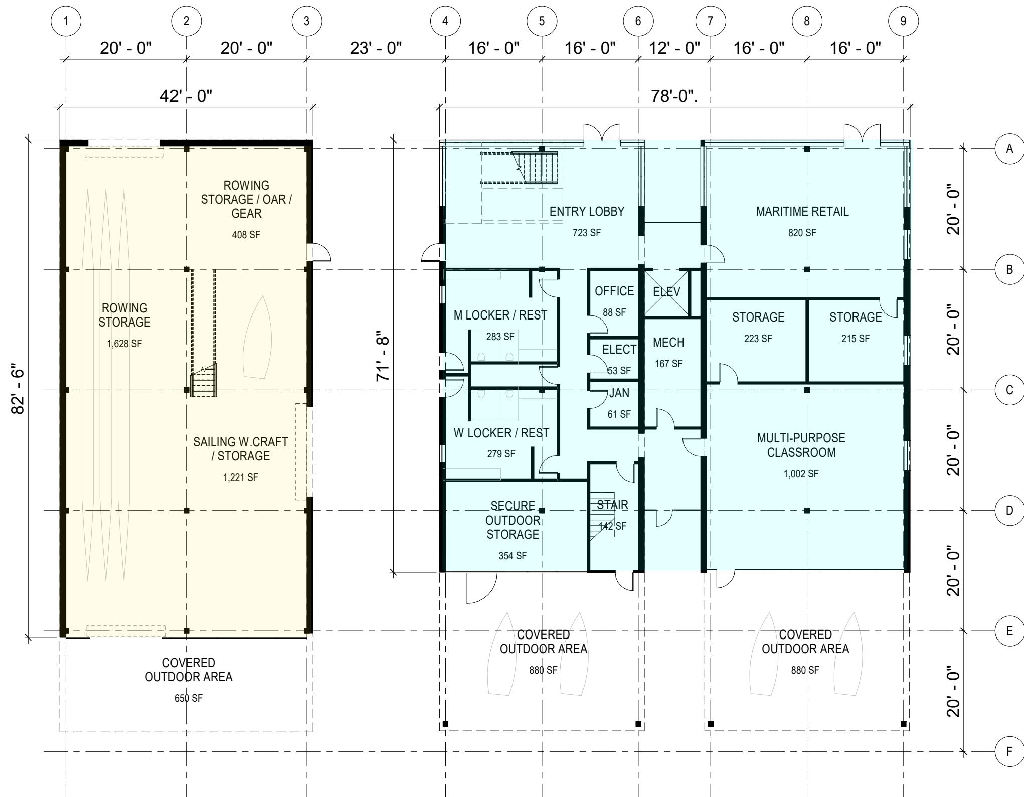
Floor Plan - Level 1
