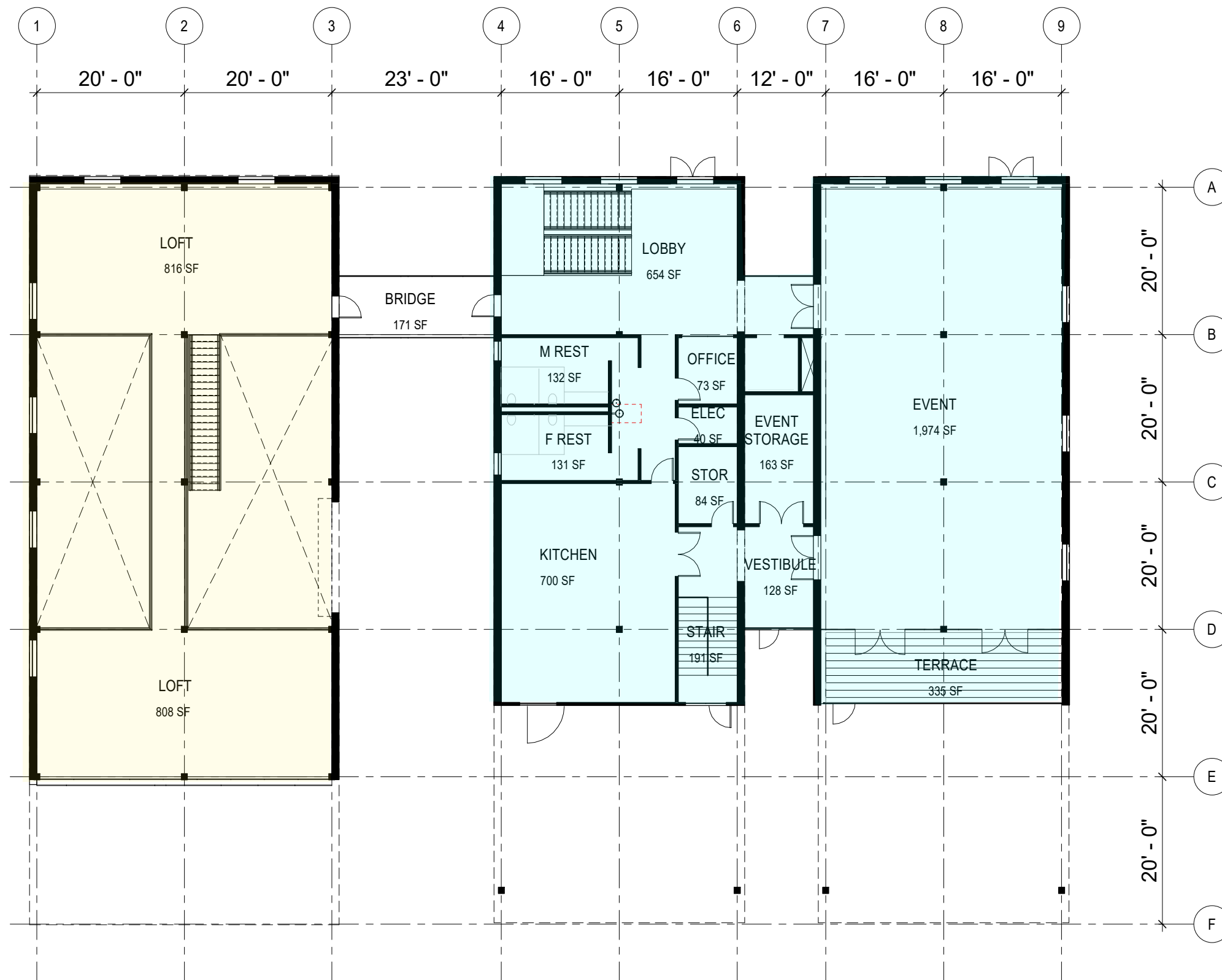
Floor Plan - Level 2
