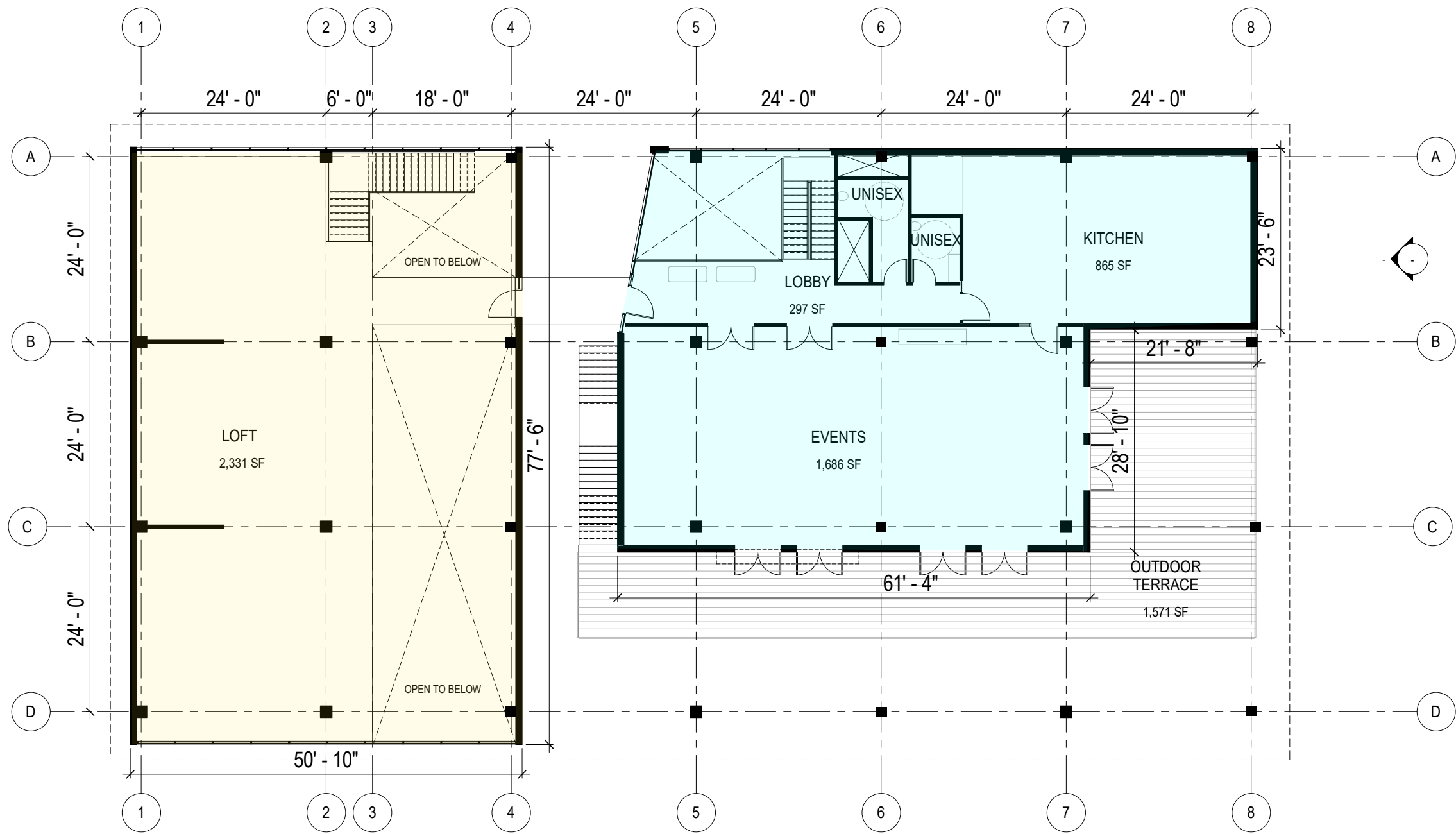
Floor Plan - Level 2
